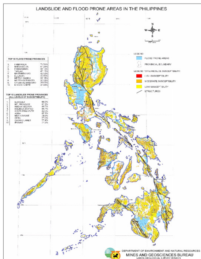
Figure 3.2.3.6: Map of landslides and flood prone areas in the Philippines 74
