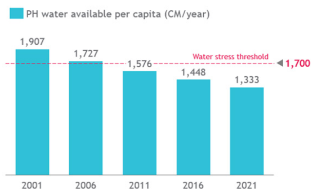
Figure 4.2.2.1. Water availability per capita, 2001-2021
