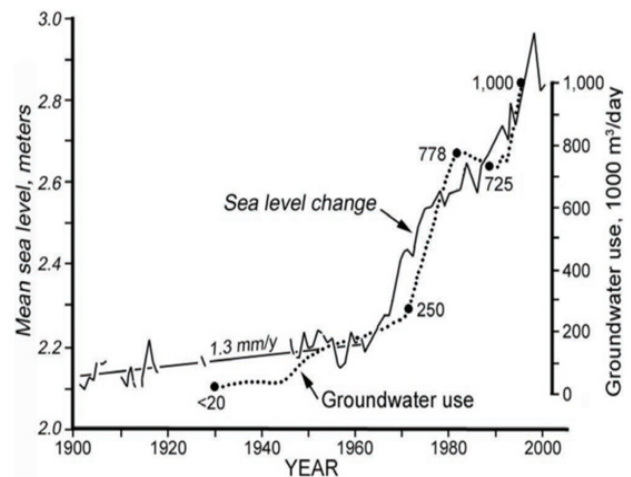
Figure 3.2.2.3: Combined plot of sea level change at Manila South Harbor and groundwater use in Metro Manila from 1902 to 2000 63
