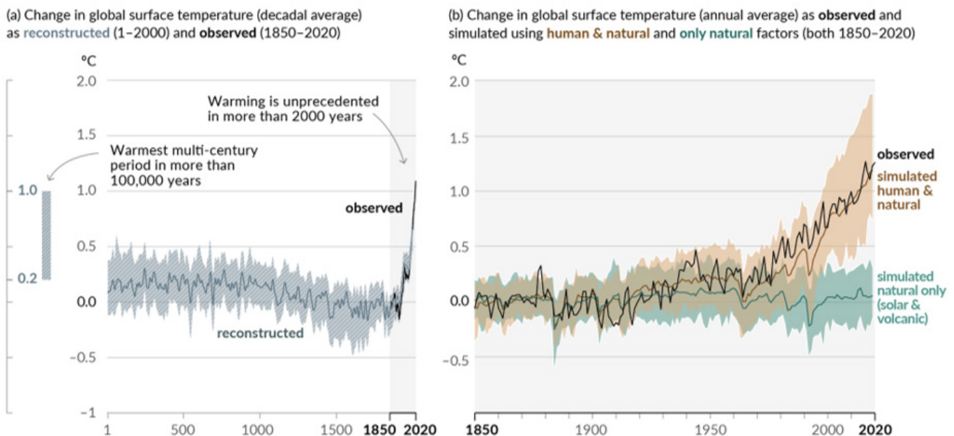
Figure 3.2.1.1: Changes in global surface temperature relative to 1850–1900 48
