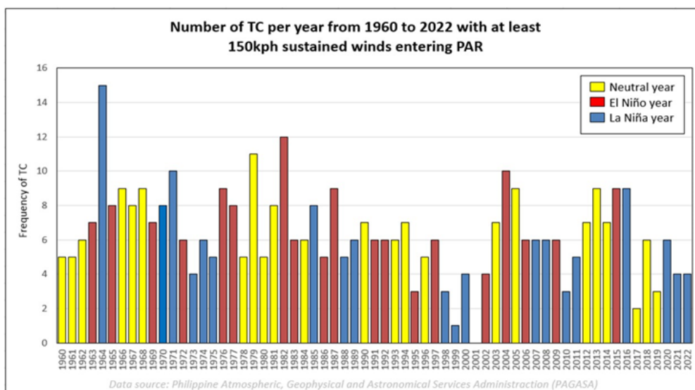
Figure 3.2.4.5: Number of typhoons per year from 1960-2022 with at least 150 kph sustained winds entering the PAR. Years are labeled according to El Niño, La Niña, or neutral conditions. Note that there were no such typhoons in 2001 85
