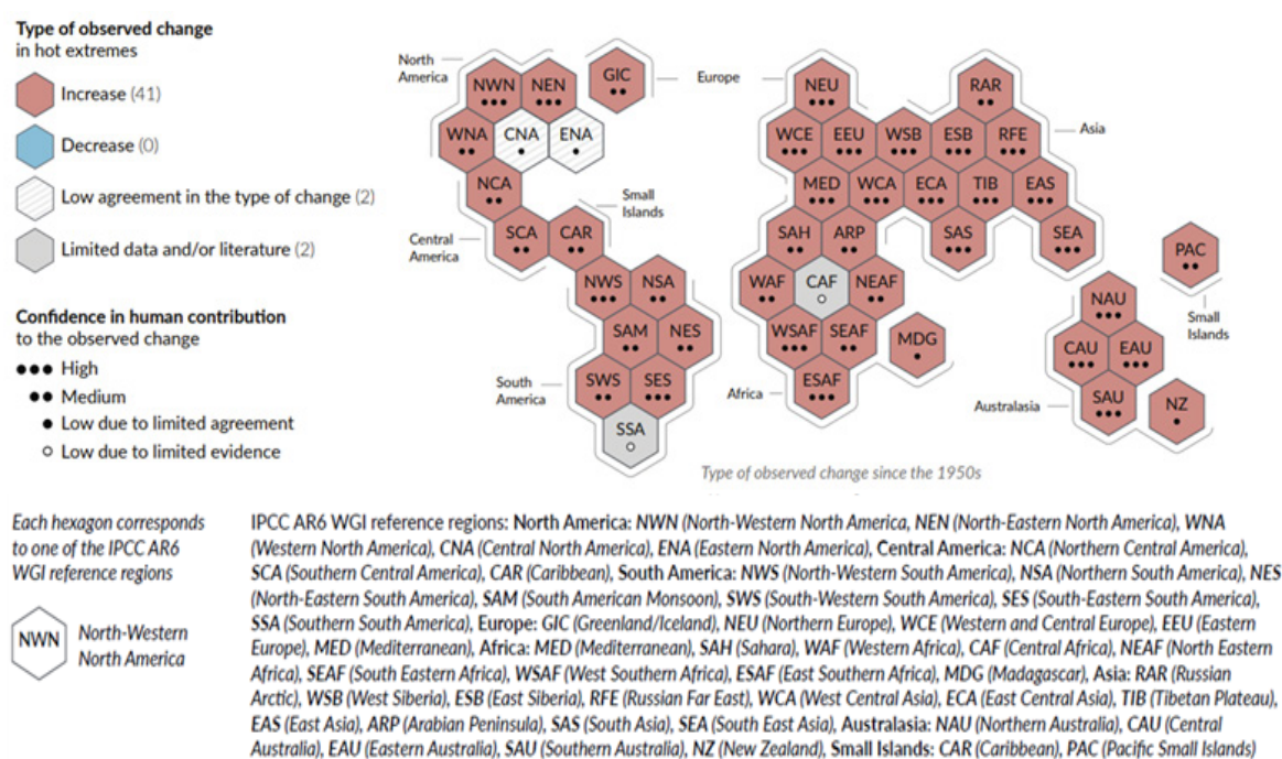
Figure 3.2.1.3: Observed change in hot extremes 51 with confidence in human contribution in each of the world's region 52
