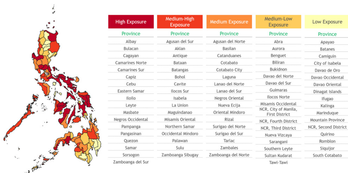
Figure 3.3.5.2 Projected provincial risk categorization between 2030-2040, SP5-8.5
