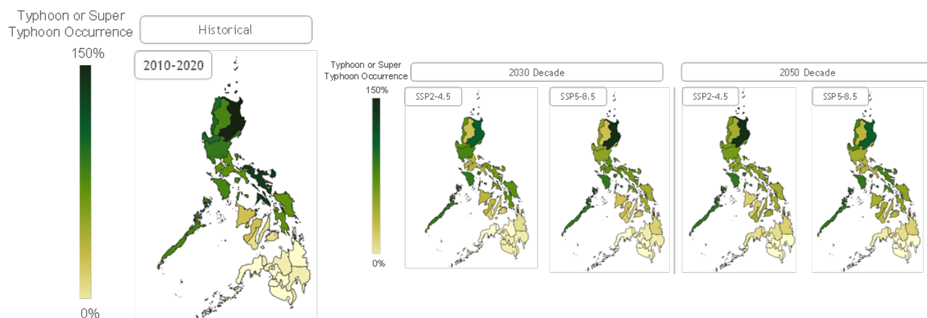
Figure 3.3.4.4: Typhoon and Super Typhoon occurrence potential by 2030 and 2050 decade 185
